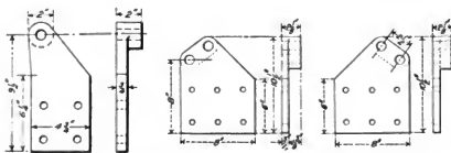
Figs. 1966-1971 Reverse Lever Quadrant Brackets for Consolidation (2-8-0) Locomotive. American Locomotive Co.
